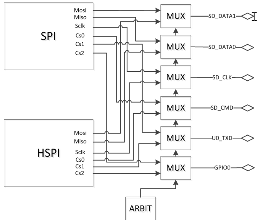
图 5-1. SPI OVERLAP 原理框图
